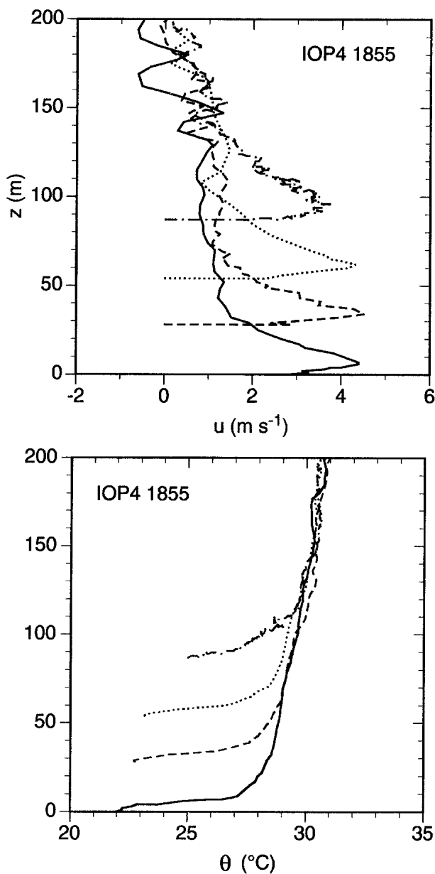
FIG. 5. As in Fig. 4, vertical profiles of (top) downslope wind speed and (bottom) potential temperature at tethersonde sites TS1–TS4 during IOP4 at 1855 MST. The vertical axis indicates height above the surface at the lowermost site (TS1). TS4 is the dashed–dotted curve.
